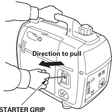
STARTER GRIP
