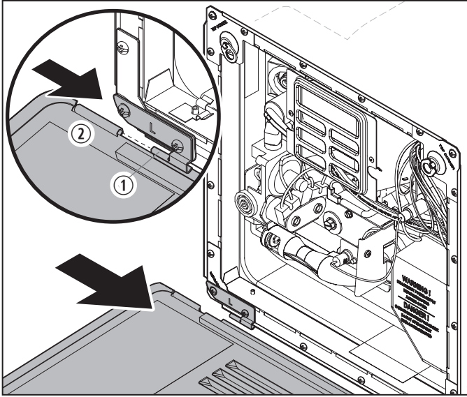
15 Sliding the Access Door onto the Left Hinge Bracket
