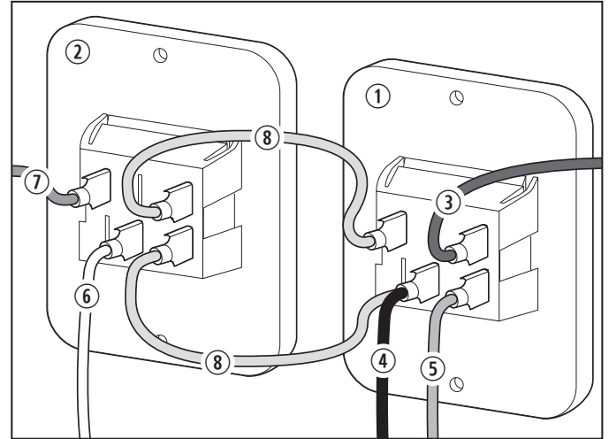
11 Single Combination Switch Wiring
