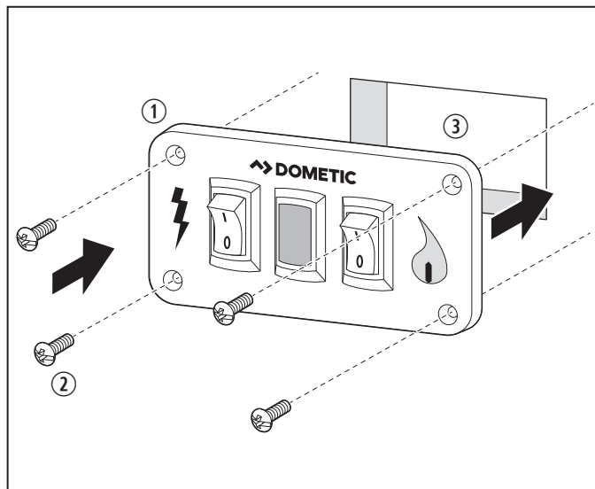
9 Installing the Dual Switch
