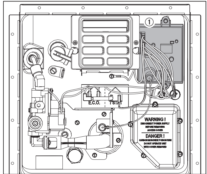
22 DSI control board
