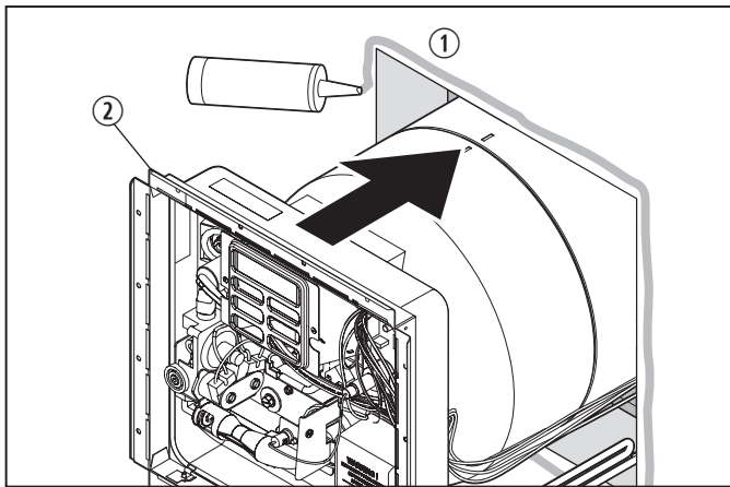
13 Caulking the Unit
