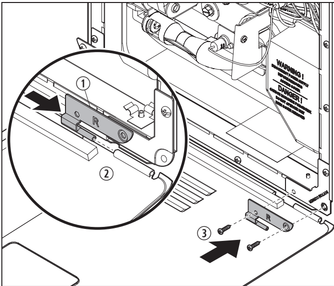
16 Attaching the Right Hinge Bracket
