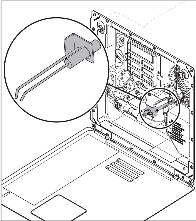
21 Inspecting the Electrode
