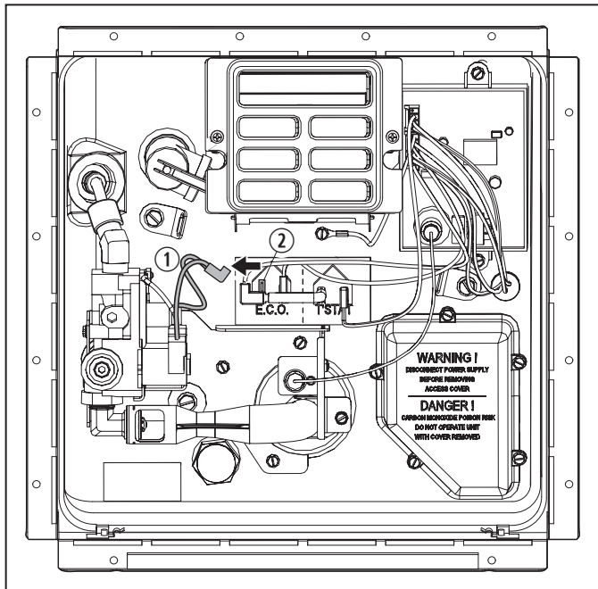
18 Removing the Red Wire from the E.C.O. Switch
