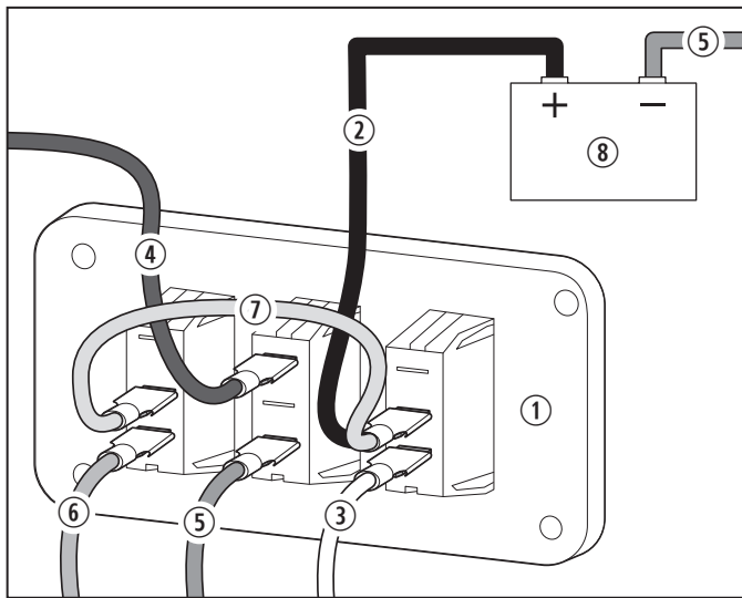
12 Dual Switch Wiring
