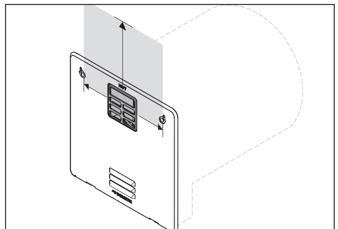
4 Vent Clearances
