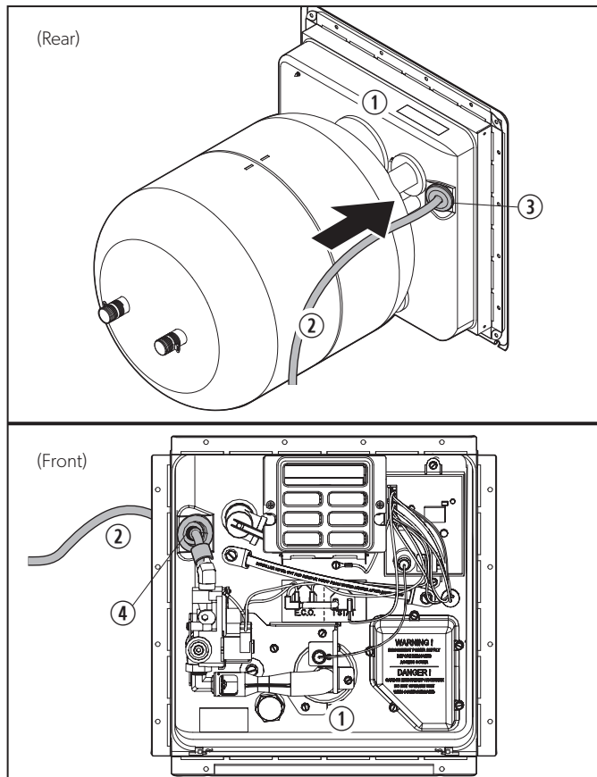
7 Sealing the Gas Line Opening With the Grommet
