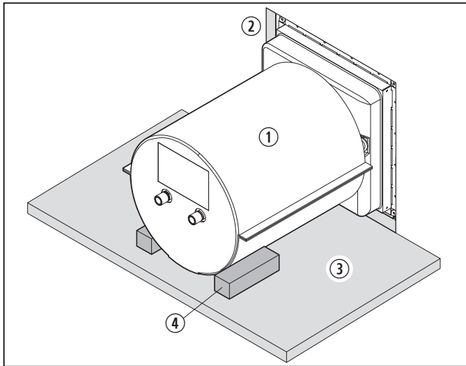
5 Blocking the Water Heater
