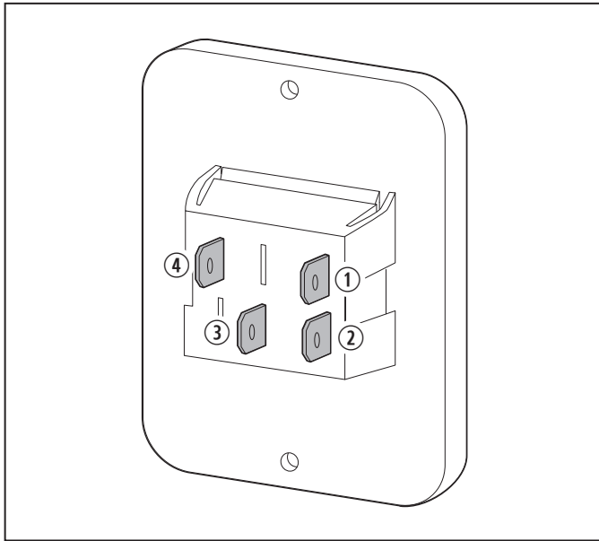
10 Control Switch Wiring
