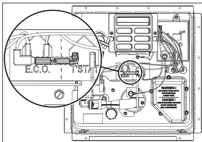
19 Thermal Cut-off
