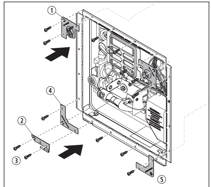
14 Securing the Brackets to the Water Heater Flange
