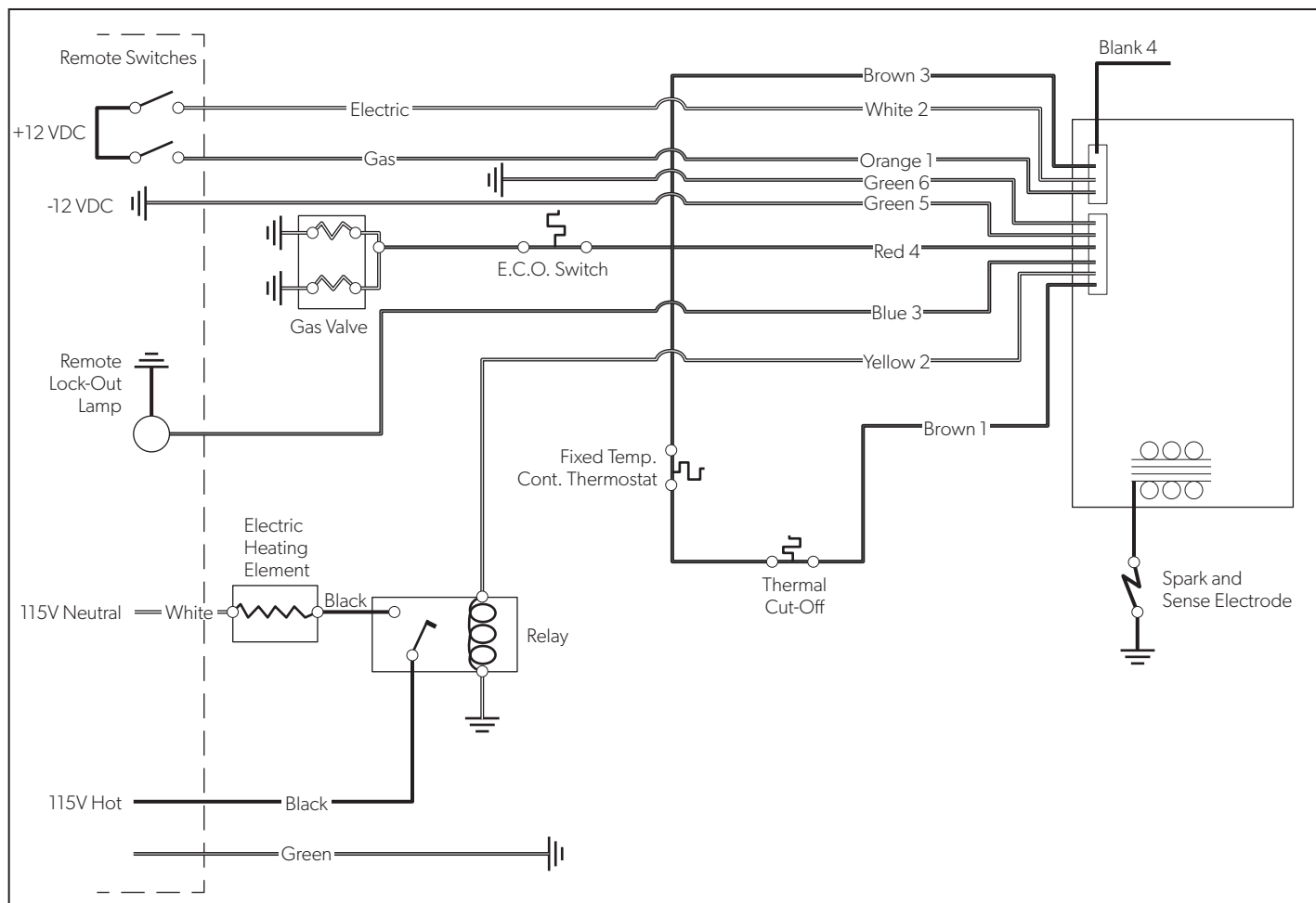
24 Combination Gas/Electric
