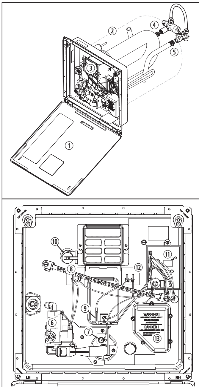
2 WH - 10GEA and WH - 16GEA Component Locations
